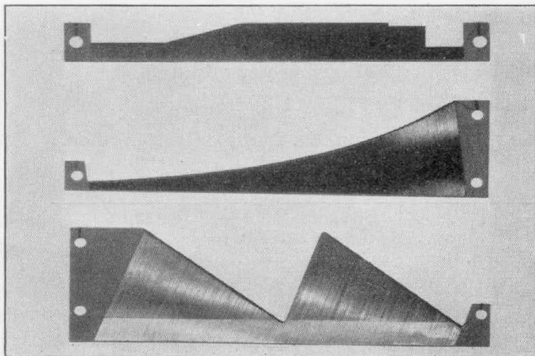
Figure 4. Three types of mandrels shaped to give desired resistance variations. At the foot is a double sawtooth, in the center a logarithmic, and at the top a combination of shapes.
