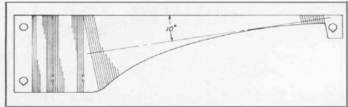
Figure 7. A combination mandrel, on which the curved portion is wound with a single kind of wire and the straight portion with several different kinds to approximate the desired characteristic.
