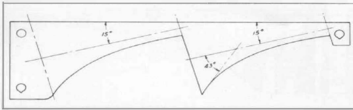
Figure 6. Double logarithmic mandrel for 30-db range.
