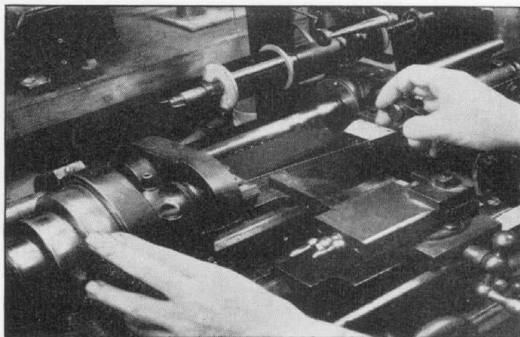
Figure 9. Hand winding, as shown here, is often used on steeply sloping mandrels.
