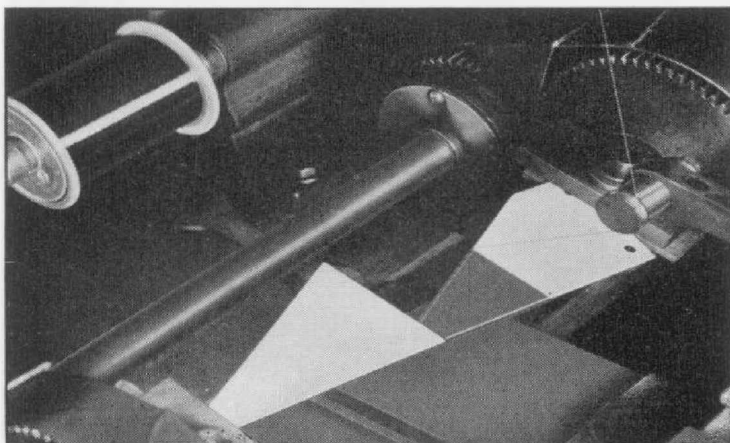
Figure 8. Close-up of the double sawtooth during winding, showing how the mandrel is clamped in the lathe.
