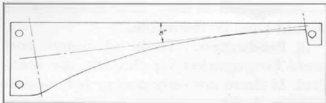
Figure 10. Mandrel widths are laid out perpendicular to the winding axis as shown here by the center line.
