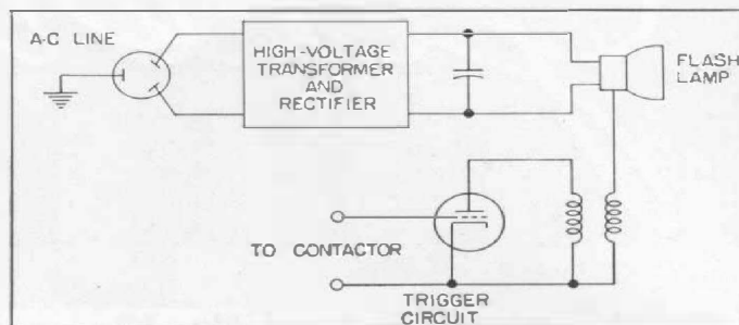
Figure 3. Functional circuit diagram of the Strobolume.
